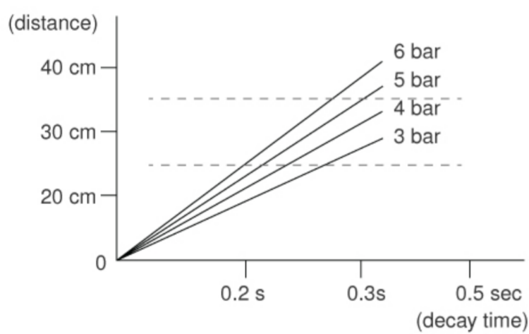
*Decay Time ( ±1,000v→±100v )
