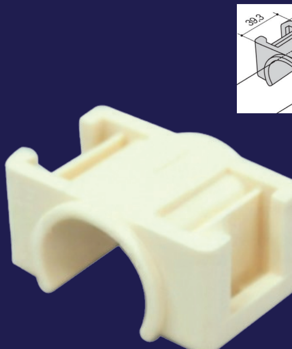
Housing Pin (Double) P/N: KH102-PC200D
